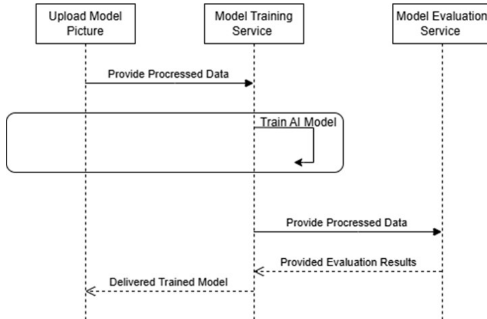
Fig 4.3.1 Sequence diagram
