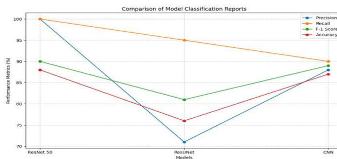
Fig 5.2.1 – Visualization of comparison of models
